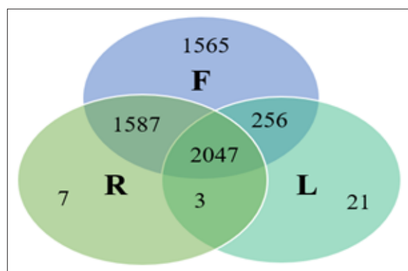
Figure 1. Venn diagram of implemented models for dataset 1.
